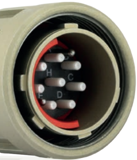
838 ELIO® 8 contacts Screw coupling Coding by ring orientation
